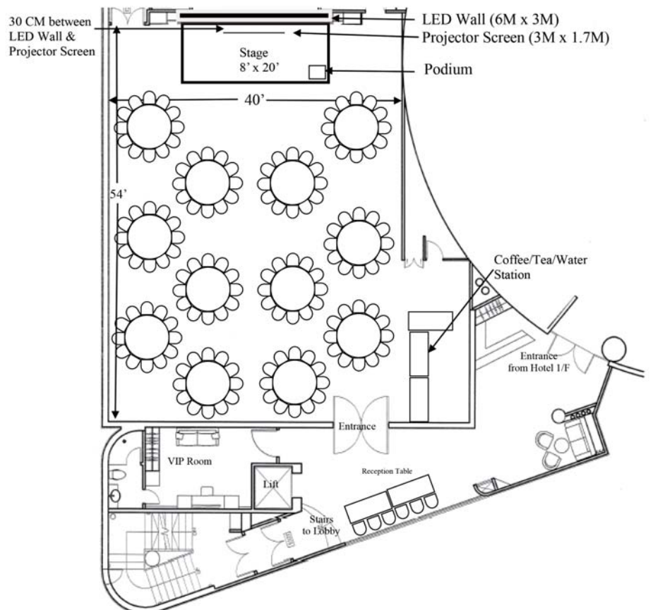
Ballroom Floor Plan 宴會廳平面圖
